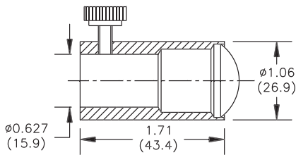
A08084 Spot Lens
