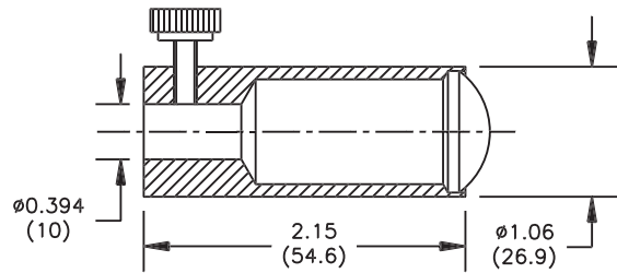
A08082 Small Spot Lens
