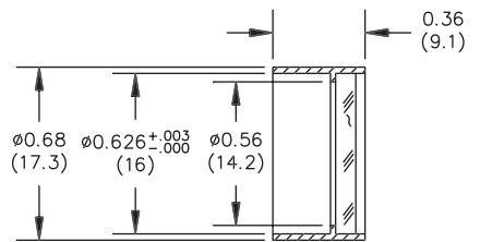
A08087 Input Opal Diffuser
