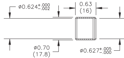
A08090 Polarizing Cap
