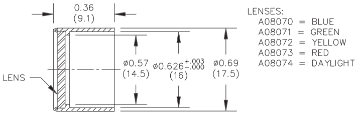
A08931 Color Filter Adapter
