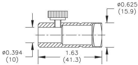
A08080 Spot Lens
